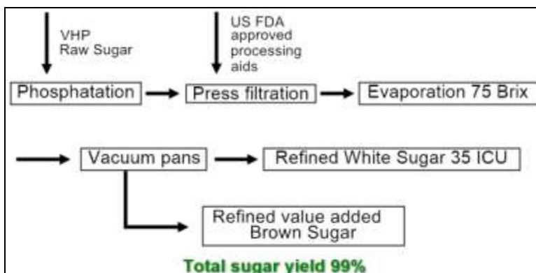
Figure 1 depicts the simplified refining process selected:
